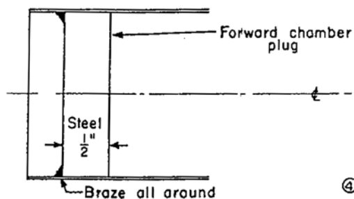
Figure 6. Typical nozzle and plug constructions.
