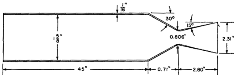
Figure 7. Engine dimension.
